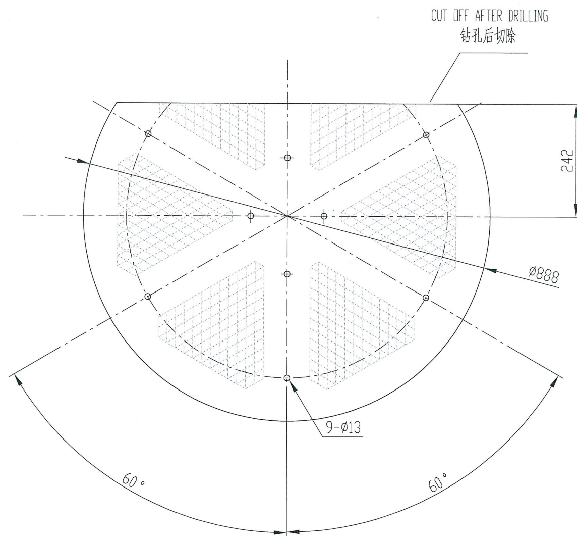
DETAIL DRAWING OF DRILLING 钻孔详图
