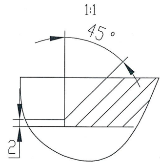
DRAWING OF OPENING GROOVE 开孔坡口图
