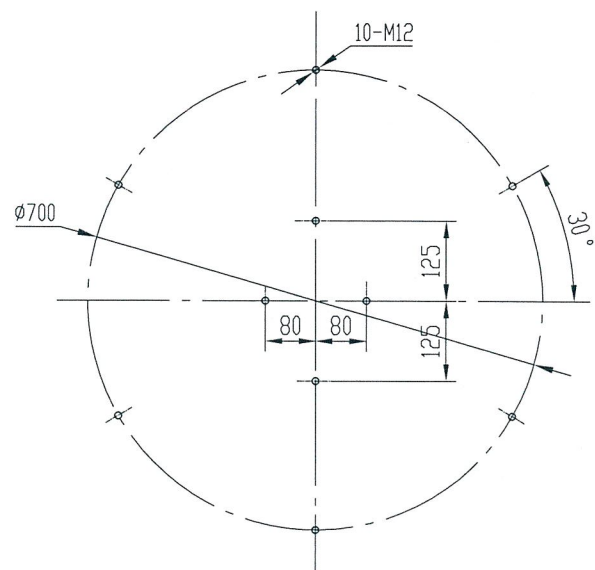
TIE ROD POSITION AT VIEW A A向拉杆孔位置
