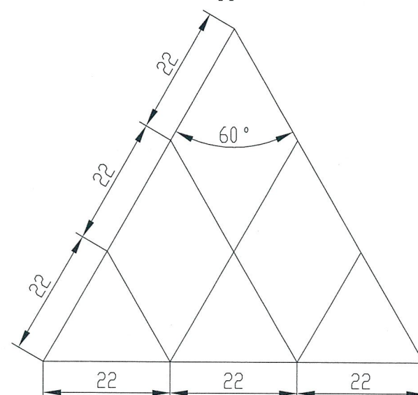
DETAIL DRAWING OF TUBE PITCH 孔距详图
