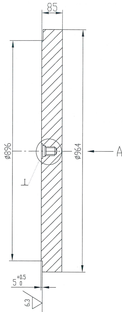
TIE ROD POSITION AT VIEW A A向拉杆孔位置
