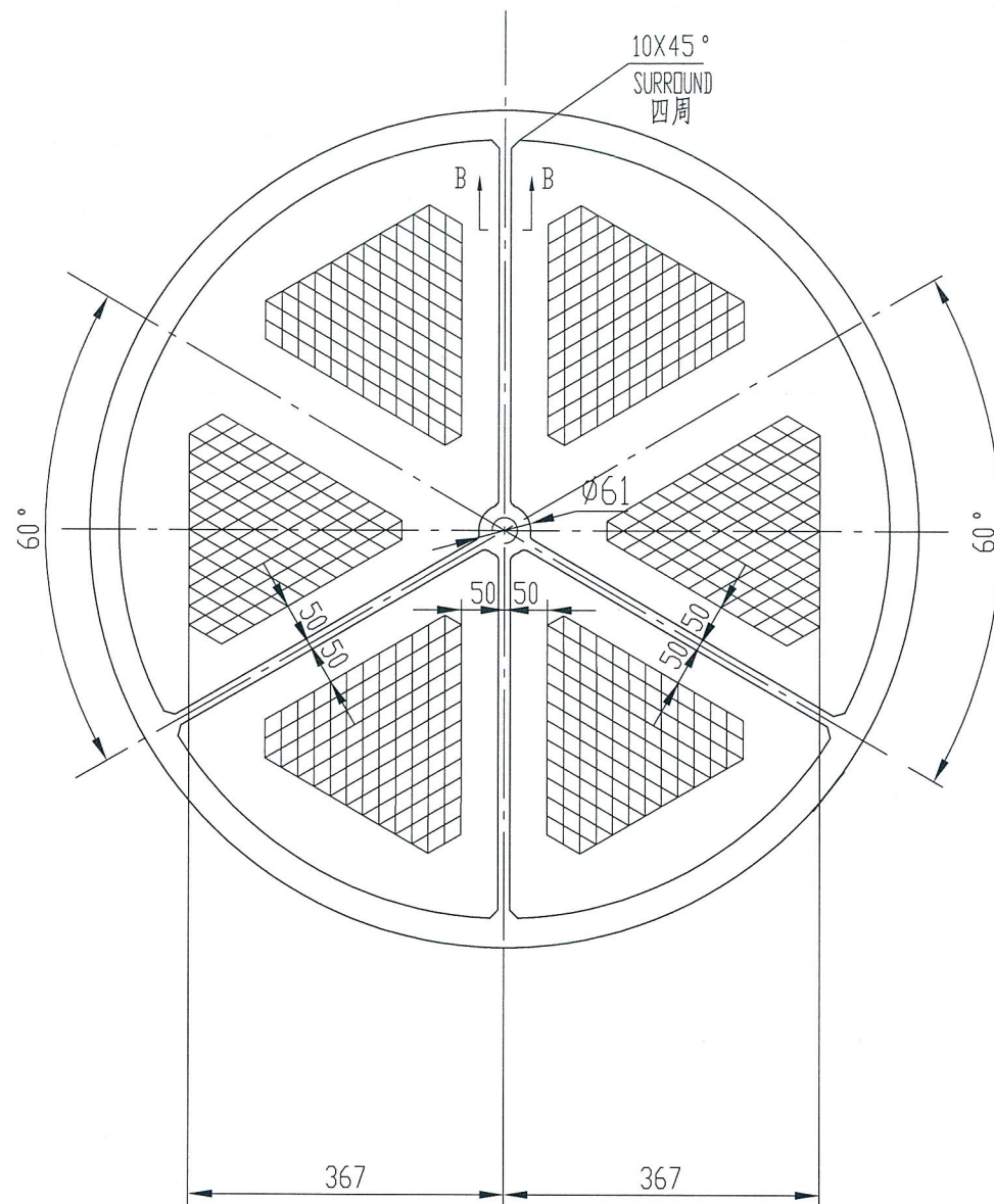
TIE ROD POSITION AT VIEW A A向拉杆孔位置
