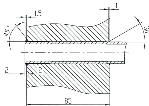
DETAIL DRAWING OF TUBE WELDING 换热管焊接详图
